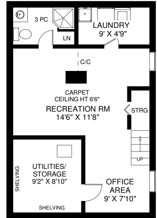
LOWER FLOOR APPROXIMATELY 599 SQ FT
